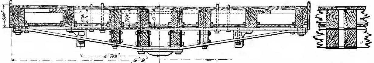
Fig. 1453. Cross Section of Bolster.
